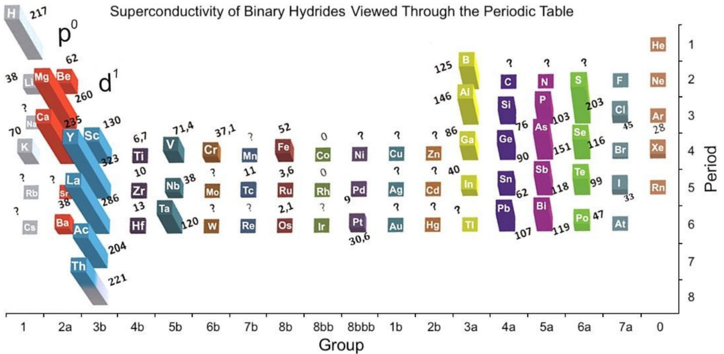
Mendeleev table with already investigated binary XH_n , where the numbers are maximum calculated T_c .
